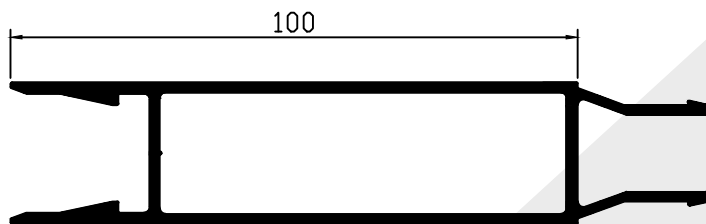
HP44A HP44M
